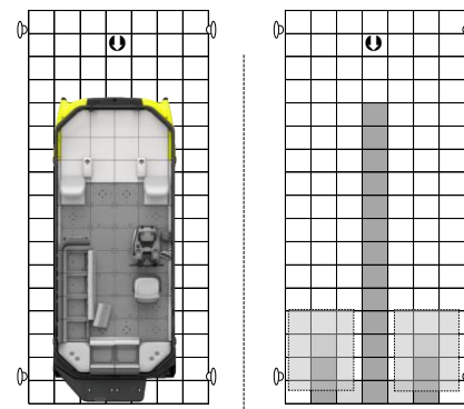
UNIVERSAL 22ft. Sea-Doo Switch Regulated Buoyancy Cell Dock Size: 11'8" wide x 28'4" long Cubes: 119
