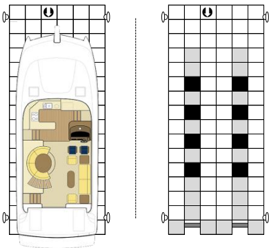
UNIVERSAL 22ft. Power Catamaran Boat Dock Distance between hulls (on center): 50-70" Size: 10' wide x 26'8" long Cubes: 86 Item No.: D60-16-PC-000
