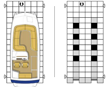
UNIVERSAL 20ft. Power Catamaran Boat Dock Distance between hulls (on center): 50-70" Size: 10' wide x 25' long Cubes: 80 Item No.: D60-15-PC-000
