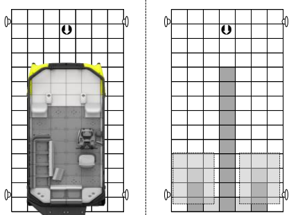
UNIVERSAL 18ft. Sea-Doo Switch Regulated Buoyancy Cell Dock Size: 11'8" wide x 23'4" long Cubes: 98
