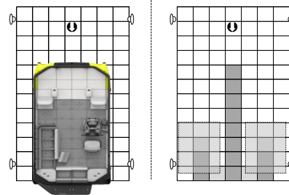
UNIVERSAL 13ft. Sea-Doo Switch Regulated Buoyancy Cell Dock Size: 11'8" wide x 20' long Cubes: 84
