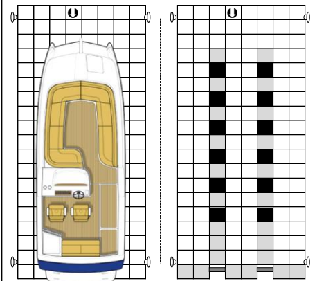
UNIVERSAL 28ft. Power Catamaran Boat Dock Distance between hulls (on center): 50-70" Size: 13'4" wide x 31'8" long Cubes: 138 Item No.: D60-19-PC-000
