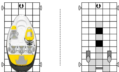
UNIVERSAL 16ft. Boat Dock Size: 8'4" wide x 18'4" long Cubes: 52 Item No.: D01-06-CC-000
