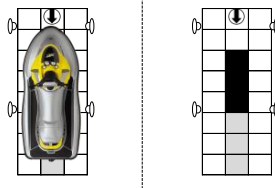
UNIVERSAL P.W.C. Dock Size: 60" wide x 160" long Cubes: 21 Item No.: D01-02-CC-000
