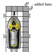
UNIVERSAL HD P.W.C. Dock (With added bow and starboard lane) Size: 80" wide x 180" long Cubes: 34 Item No.: D01-02-HD-011
