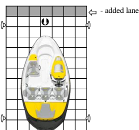
UNIVERSAL 16ft. Wide-Body Boat Dock (With added bow lane) Size: 11'8" wide x 20' long Cubes: 81 Item No.: D01-06-CC-111
