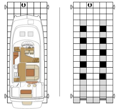
UNIVERSAL 24ft. Power Catamaran Boat Dock Distance between hulls (on center): 50-70" Size: 10' wide x 28'4" long Cubes: 90 Item No.: D60-17-PC-000
