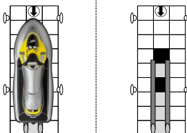
UNIVERSAL XL P.W.C. Dock Size: 60" wide x 180" long Cubes: 25 Item No.: D01-02-XL-000
