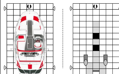
UNIVERSAL 18ft. Wide-Body Boat Dock Size: 11'8" wide x 20' long Cubes: 81 Item No.: D01-07-CC-101
