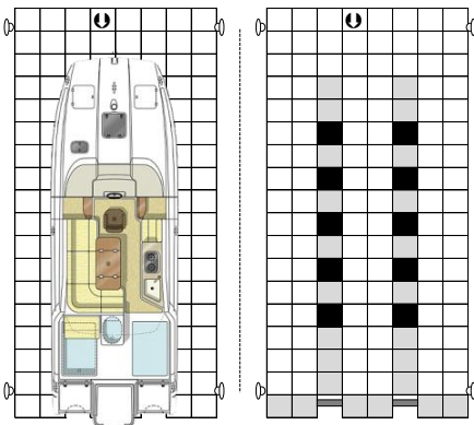
UNIVERSAL 26ft. Power Catamaran Boat Dock Distance between hulls (on center): 50-70" Size: 13'4" wide x 30' long Cubes: 132 Item No.: D60-18-PC-000
