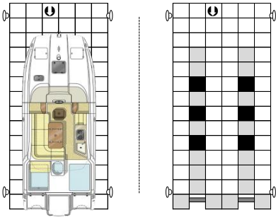
UNIVERSAL 18ft. Power Catamaran Boat Dock Distance between hulls (on center): 50-70" Size: 10' wide x 23'4" long Cubes: 76 Item No.: D60-14-PC-000
